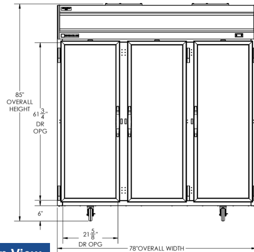
Elevation View
