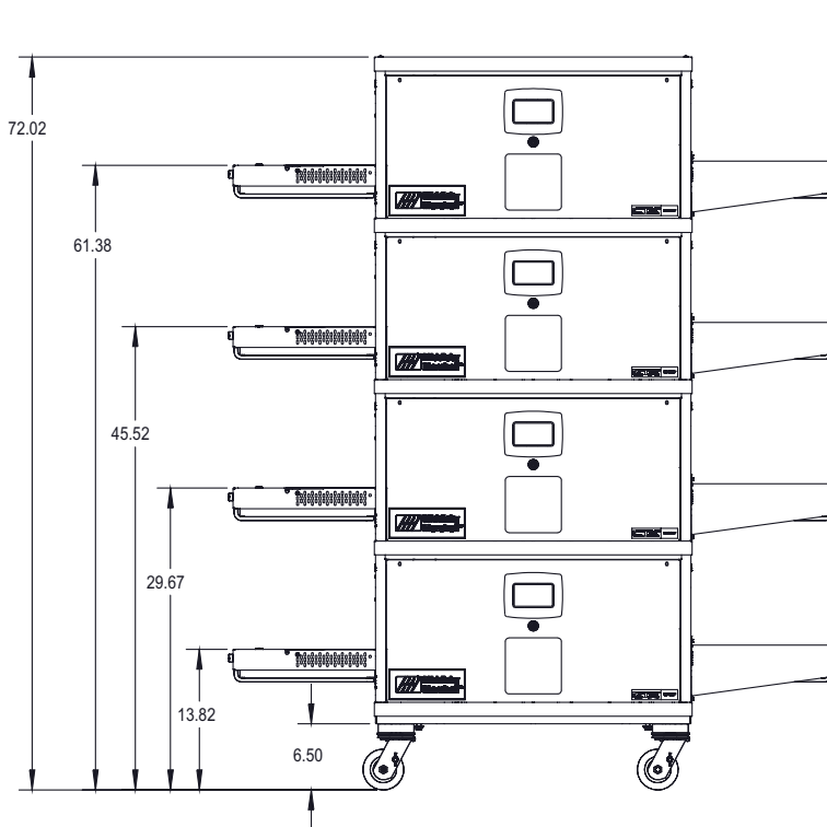
Front View – Quad Stacked with Casters
