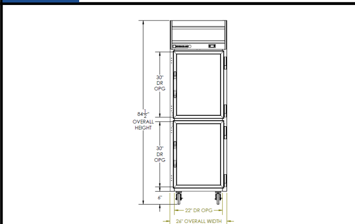
Elevation View
