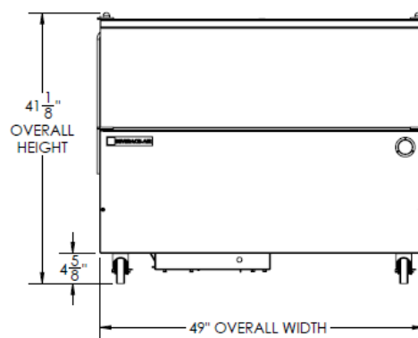
Elevation View
