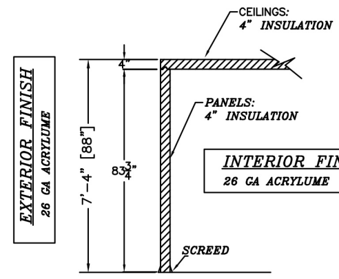
SECTION WALL WITHOUT FLOOR
