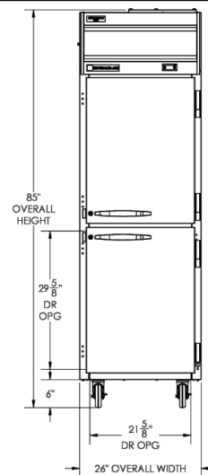
Elevation View
