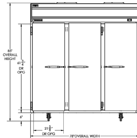
Elevation View
