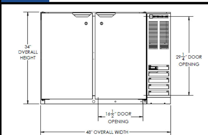
Elevation View
