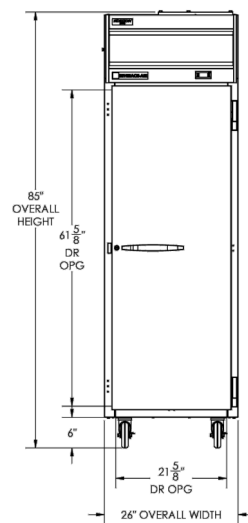
Elevation View
