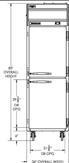
Elevation View
