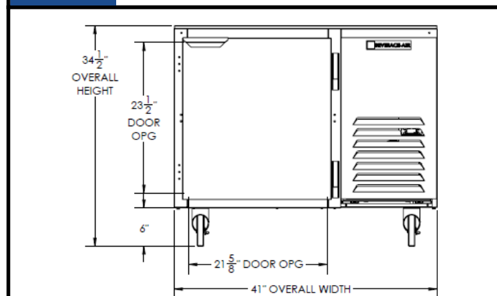
Elevation View
