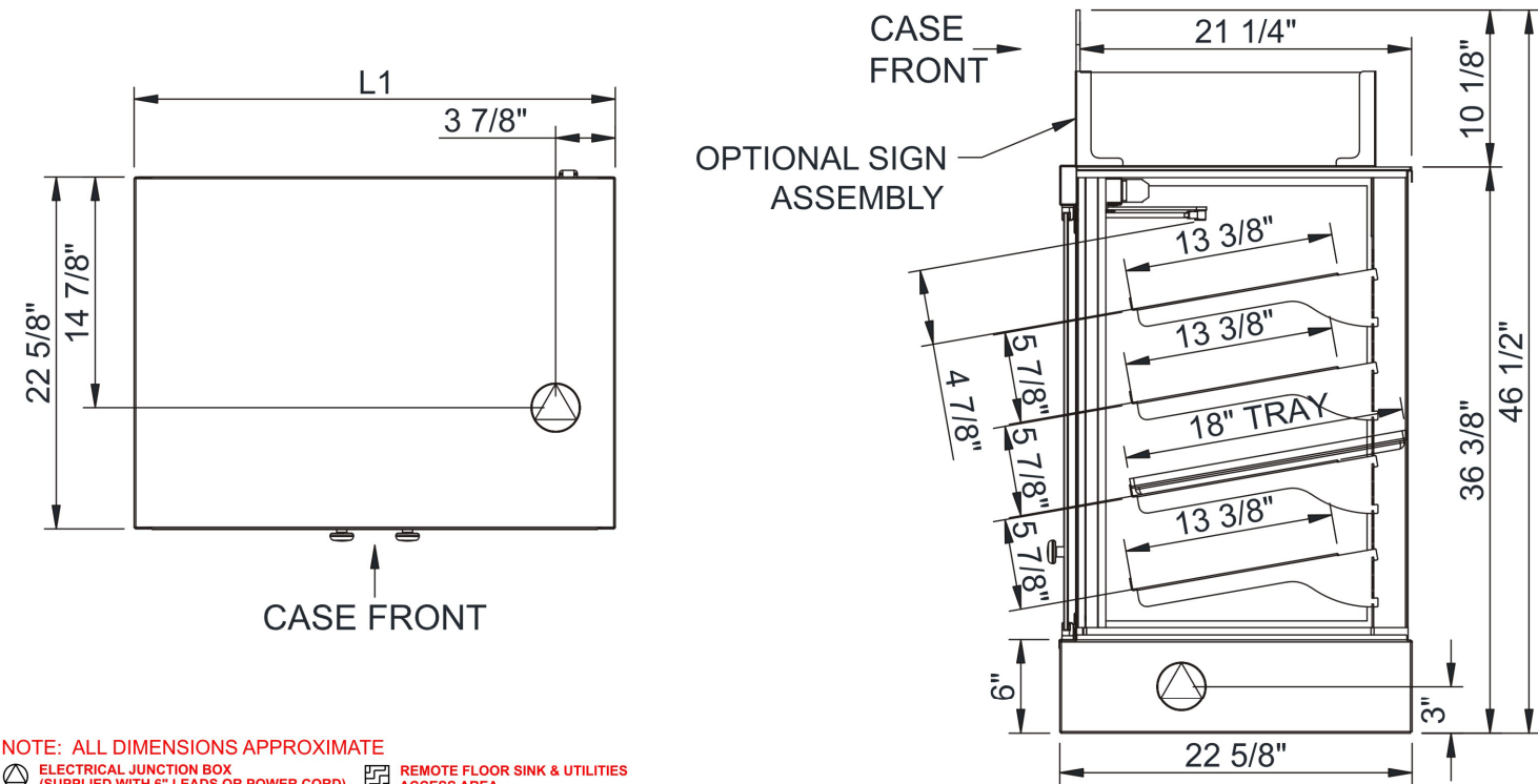
PLAN VIEW
