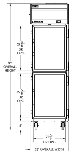
Elevation View
