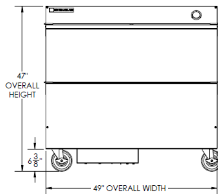
Elevation View
